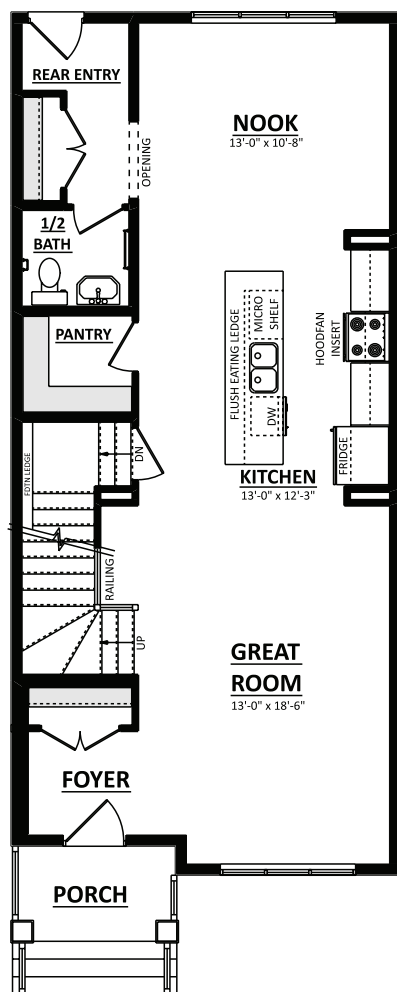
Main Floor Plan 877 Sq.Ft.
