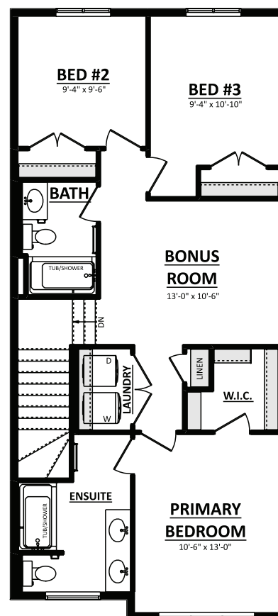
Second Floor Plan 822 Sq.Ft.
