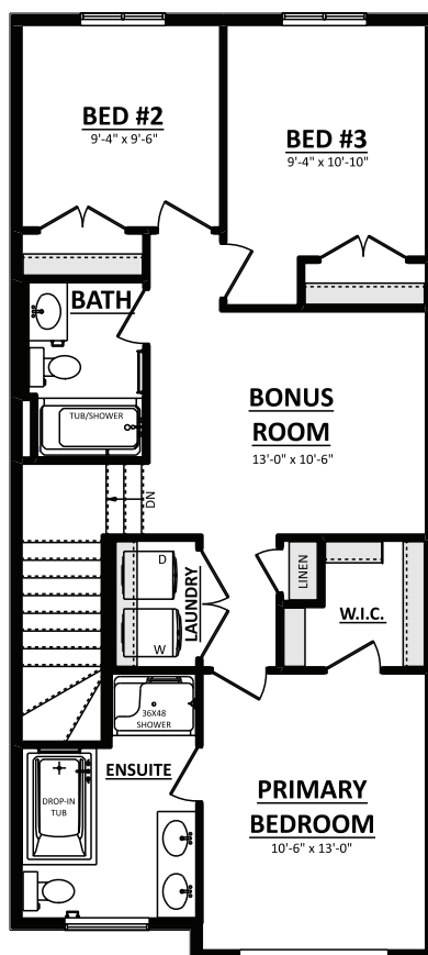
Second Floor Plan Opt. Ensuite 822 Sq.Ft.
