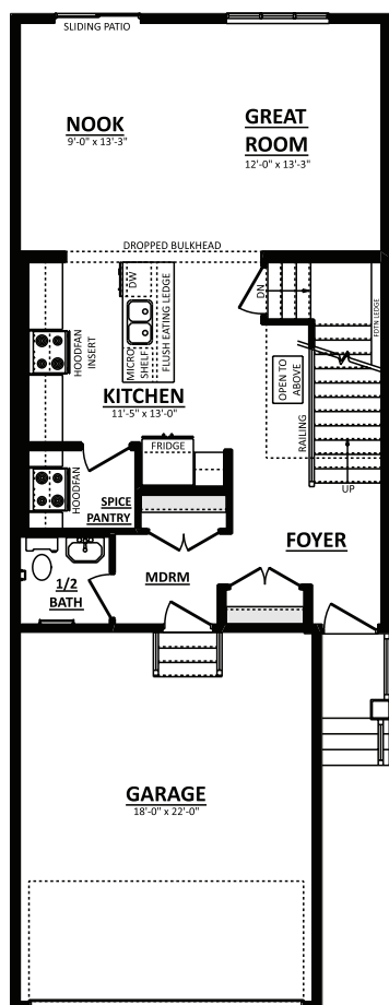
Main Floor Plan Optional Spice Pantry 792 Sq.Ft.
