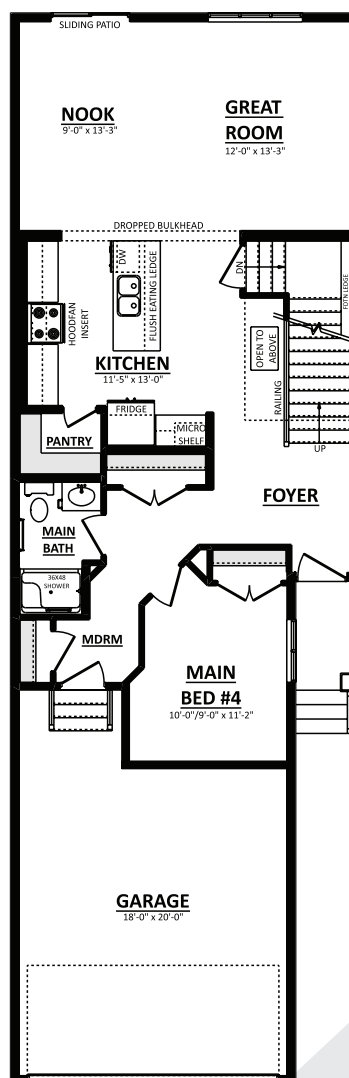
Main Floor Plan Optional Bed & Bath 973 Sq.Ft.
