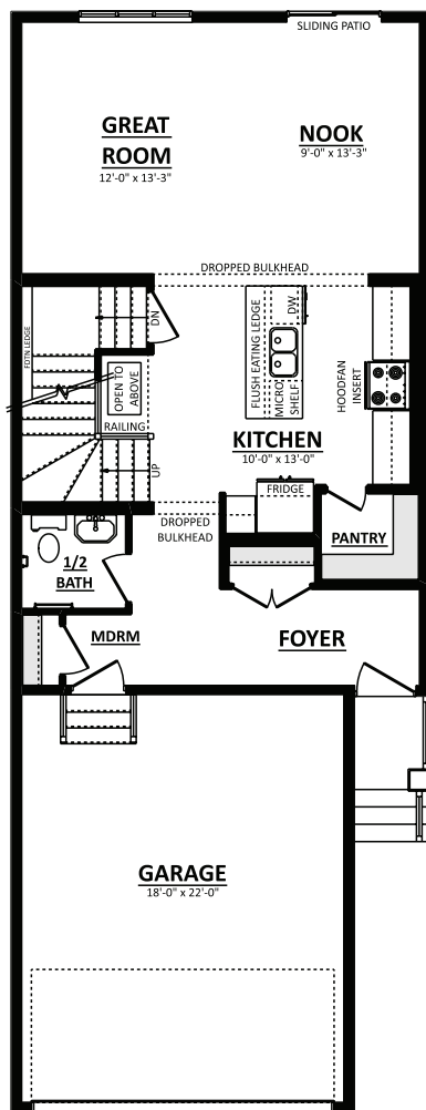
Main Floor Plan 792 Sq.Ft.
