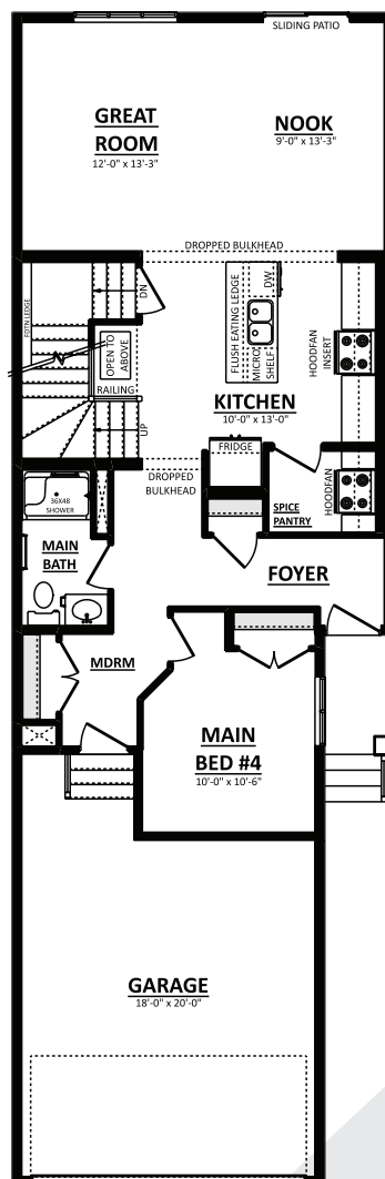
Main Floor Plan Optional Bed & Bath & Spice 973 Sq.Ft.
