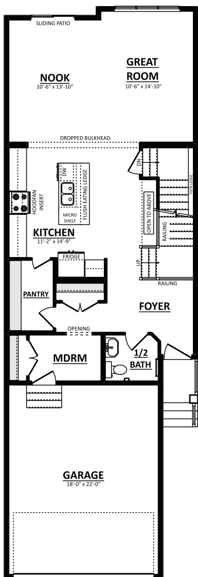
Main Floor Plan 924 Sq.Ft.
