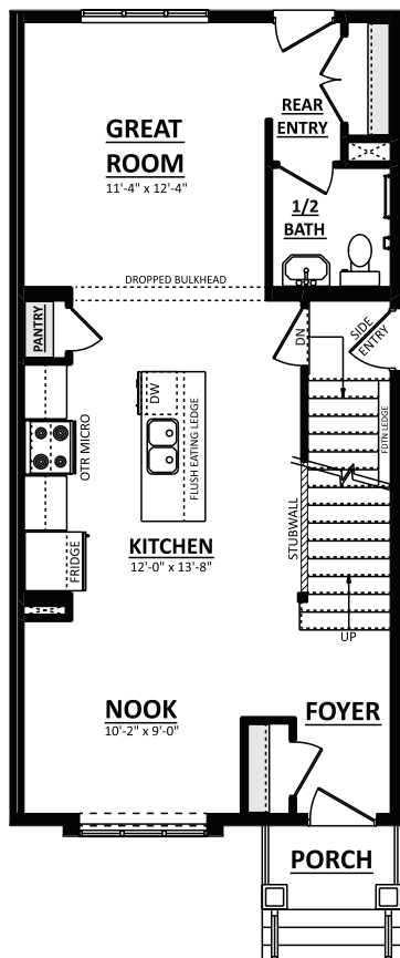
Main Floor Plan 684 Sq.Ft.
