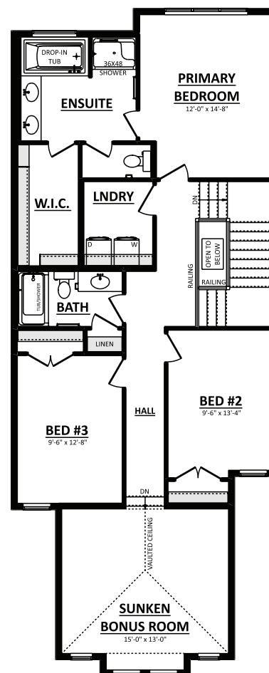
Second Floor Plan 1180 Sq.Ft.
