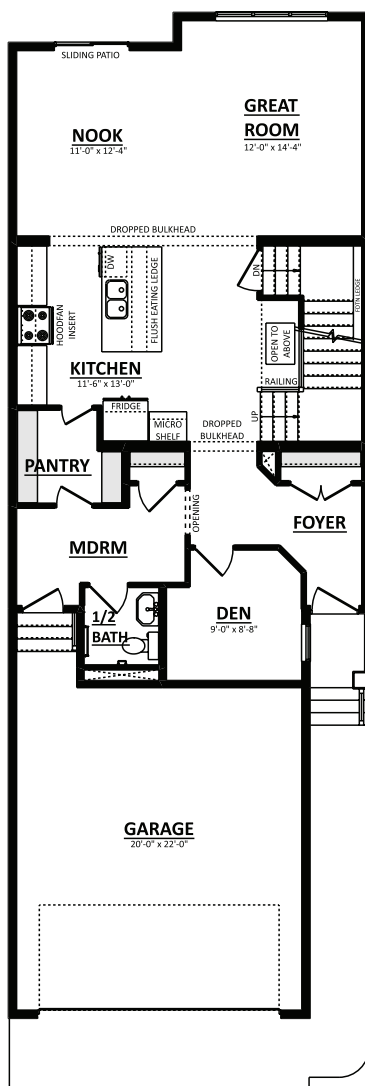
Main Floor Plan Optional Den 1016 Sq.Ft.
