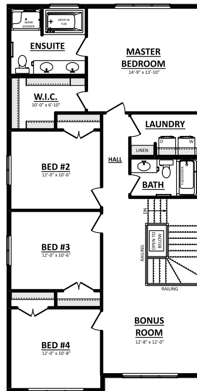
Second Floor Plan 1250 Sq.Ft.
