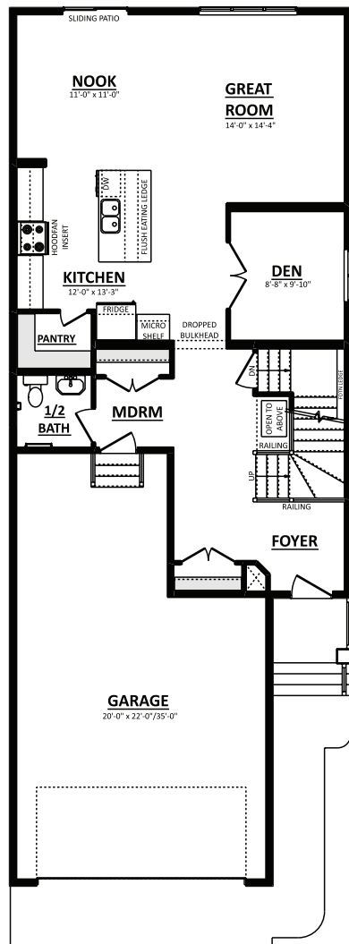
Main Floor Plan 1038 Sq.Ft.
