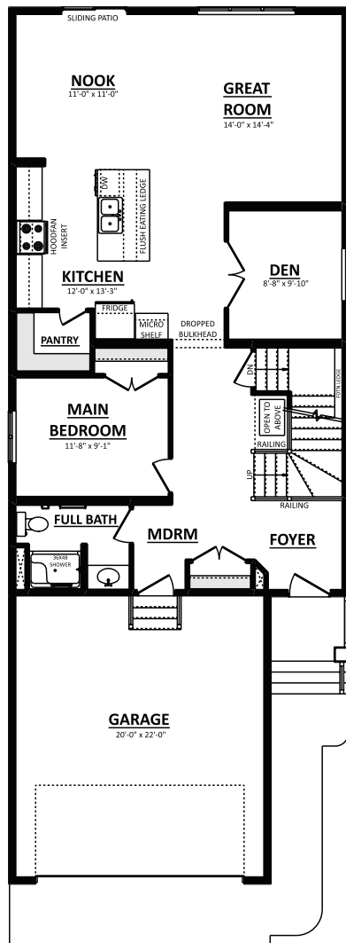
Main Floor Plan Optional Bed & Full Bath 1170 Sq.Ft.
