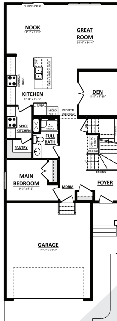
Main Floor Plan Optional Bed & Spice Kitchen 1170 Sq.Ft.
