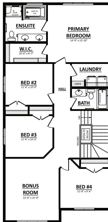
Second Floor Plan Optional Large Front Bonus 1266 Sq.Ft.
