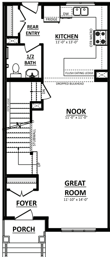
Main Floor Plan 688 Sq.Ft.
