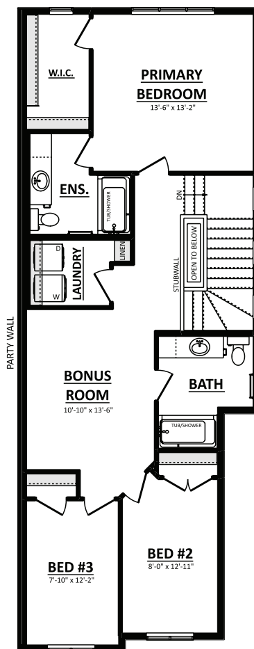
Second Floor Plan 929 Sq.Ft.
