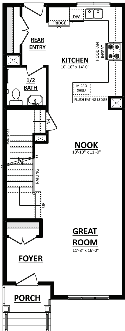
Main Floor Plan 760 Sq.Ft.
