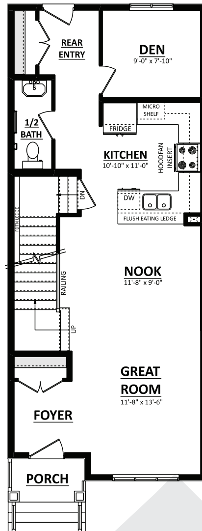
Main Floor Plan Optional Rear Den 760 Sq.Ft.
