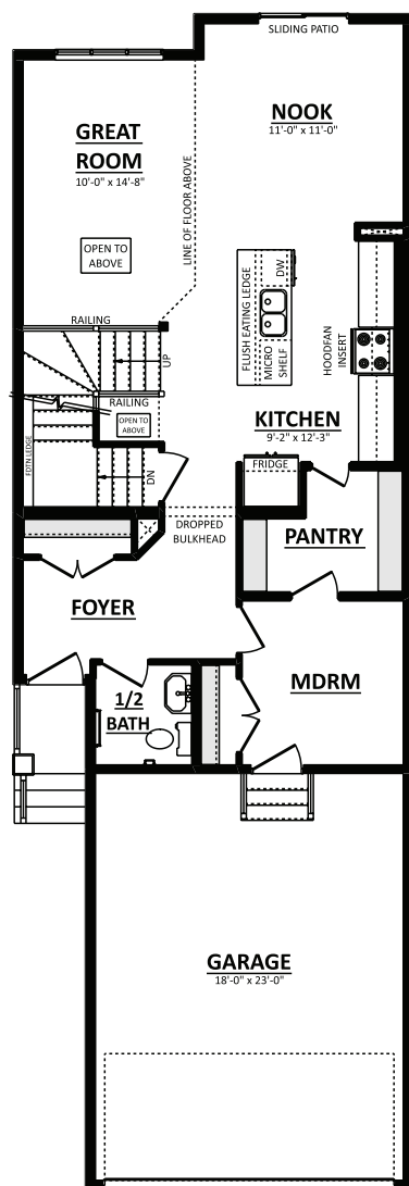
Main Floor Plan 884 Sq.Ft.
