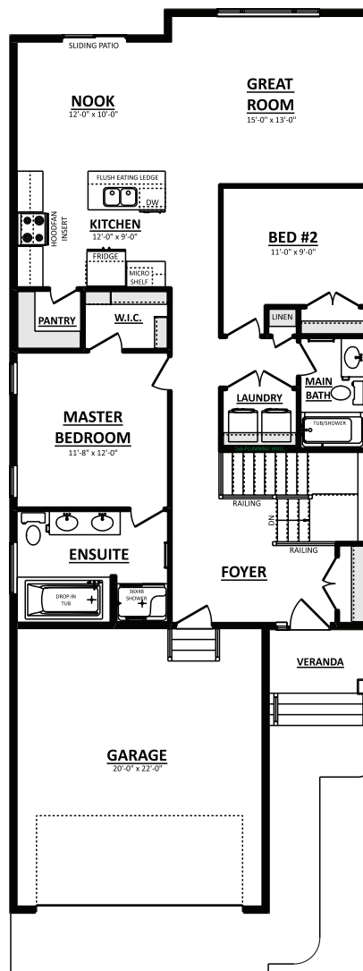
Main Floor Plan 1320 Sq.Ft.
