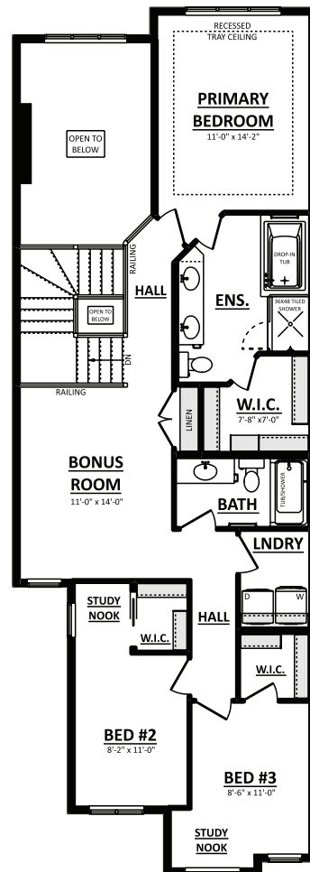
Second Floor Plan 1017 Sq.Ft.
